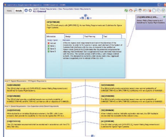
Graphical browsing of DOORS information and its traceability
